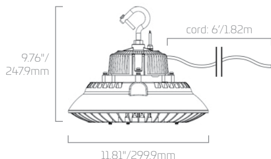
BAY 100/150W
