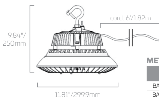
BAY 200W
